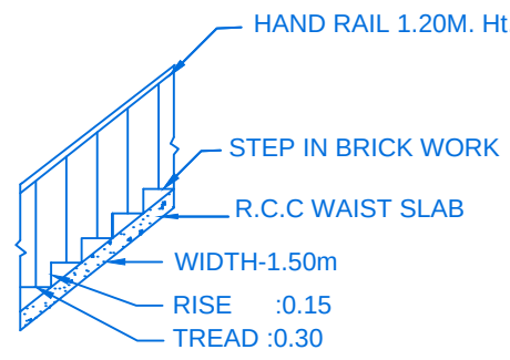
STAIR DETAIL
