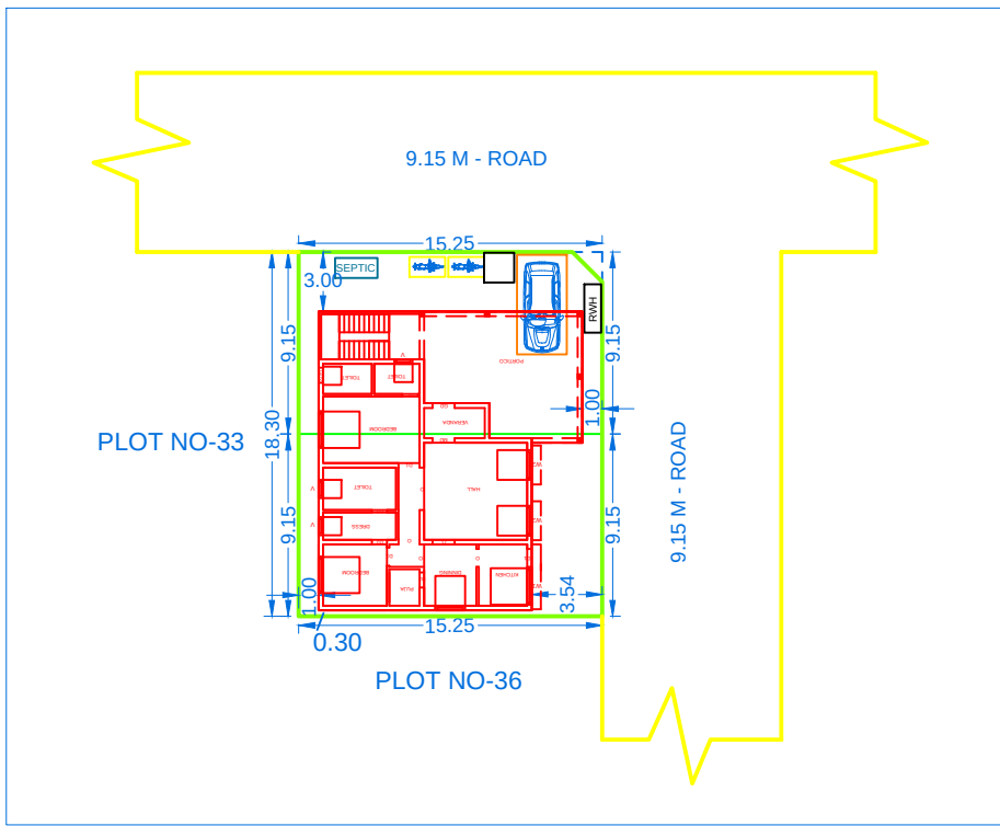
LOCATION PLAN
