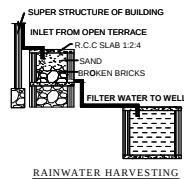
RAINWATER HARVESTING
