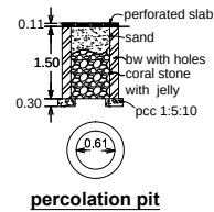
percolation pit
