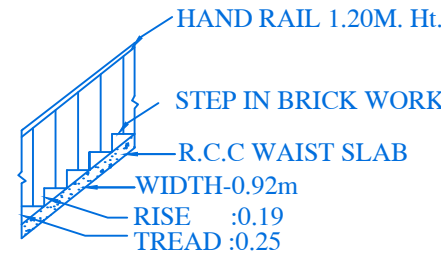
STAIR DETAIL
