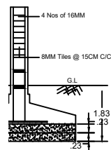
UMN DETAILS
