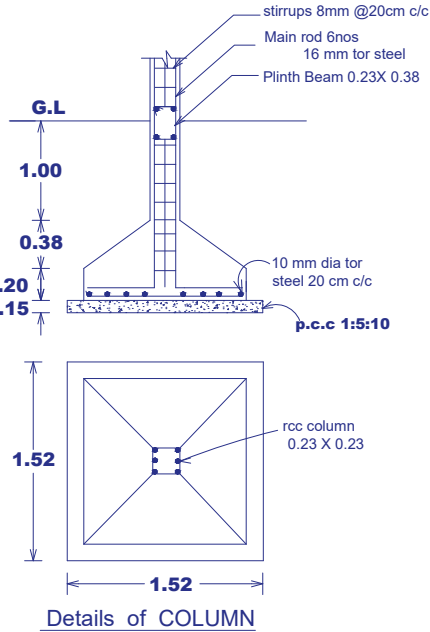
Details of COLUMN
