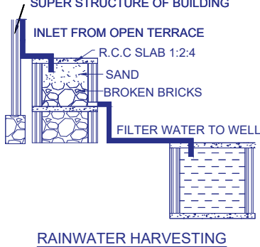
RAINWATER HARVESTING
