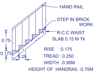
STAIR DETAILS
