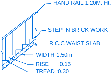
STAIR DETAIL
