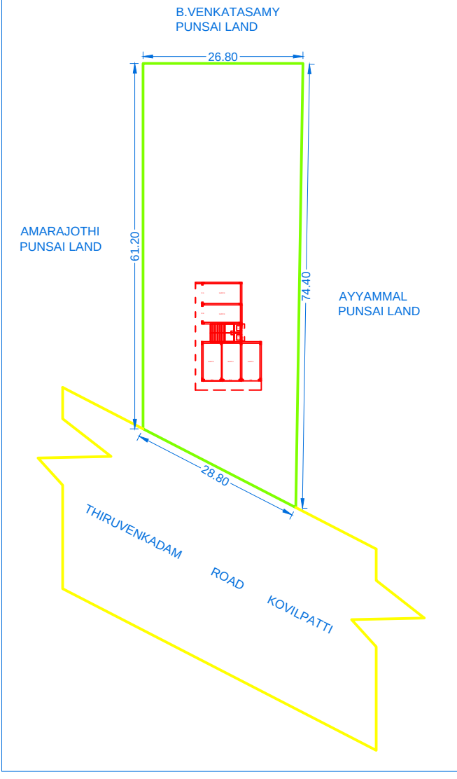
SITE PLAN
