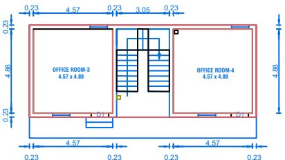
FIRST FLOOR PLAN(OFFICE ROOM)
