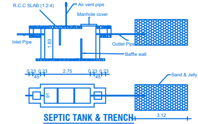
SEPTIC TANK & TRENCH
