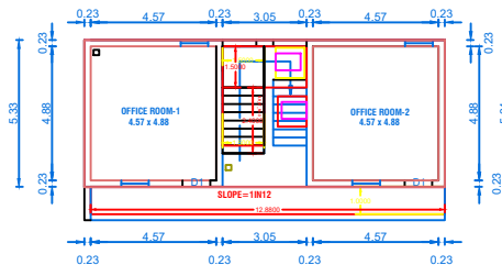
GROUND FLOOR PLAN(OFFICE ROOM)
