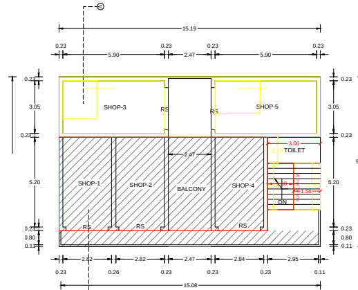
EXG & PRO.FIRST FLOOR PLAN
