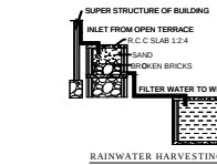
RAINWATER HARVESTING
