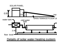
Details of solar water heating system
