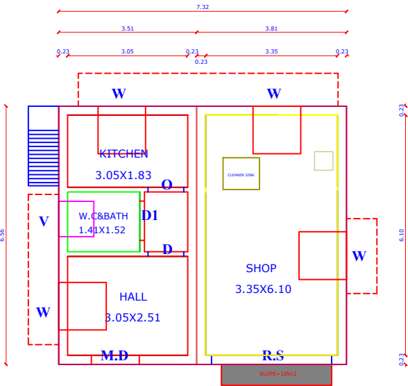
HOUSE SHOP PROPOSED GROUND FLOOR PLAN
