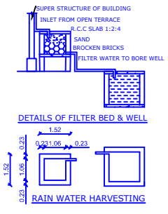
RAIN WATER HARVESTING
