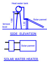
SIDE ELEVATION
