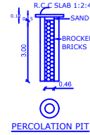
PERCOLATION PIT
