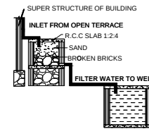
RAINWATER HARVESTING
