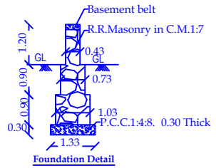
Foundation Detail
