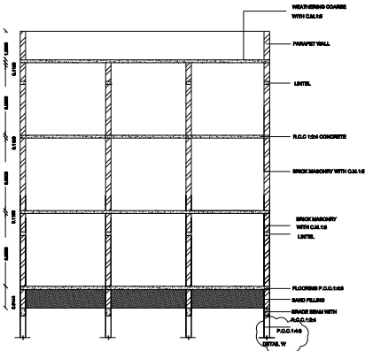
SECTION ON 'AB'
