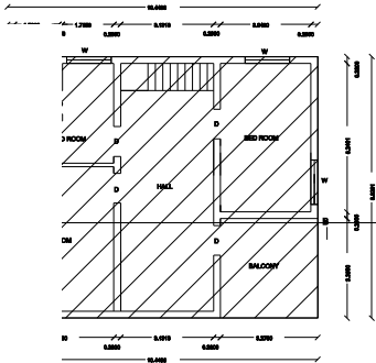
EXG F.FLOOR PLAN
