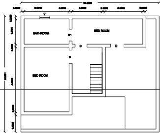
PRO S.FLOOR PLAN
