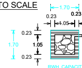
DETAILS OF FILTER BED & WELL
