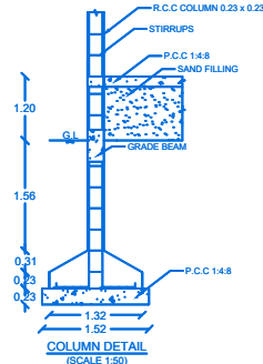
COLUMN DETAIL (SCALE 1:50)
