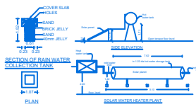
SECTION OF RAIN WATER HARVESTING TANK
