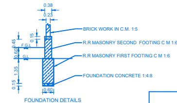
FOUNDATION DETAILS
