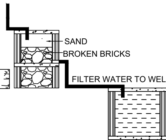
RAINWATER HARVESTING
