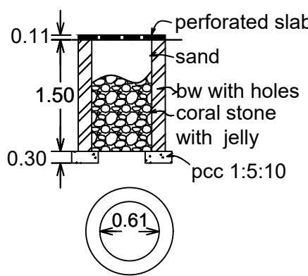
PERCOLATION PIT
