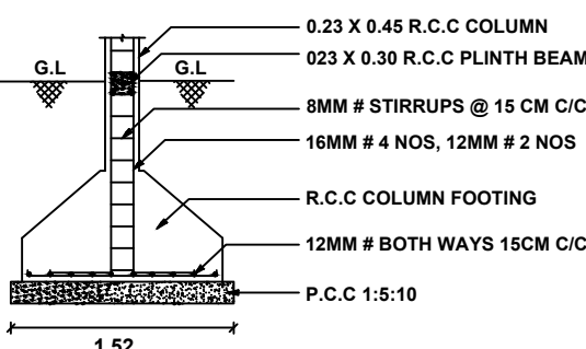
COLUMN FOOTING DETAILS
