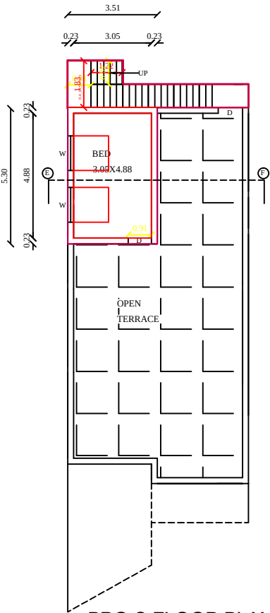
PRO.S.FLOOR PLAN
