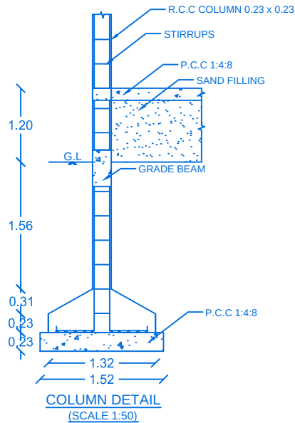
COLUMN DETAIL
