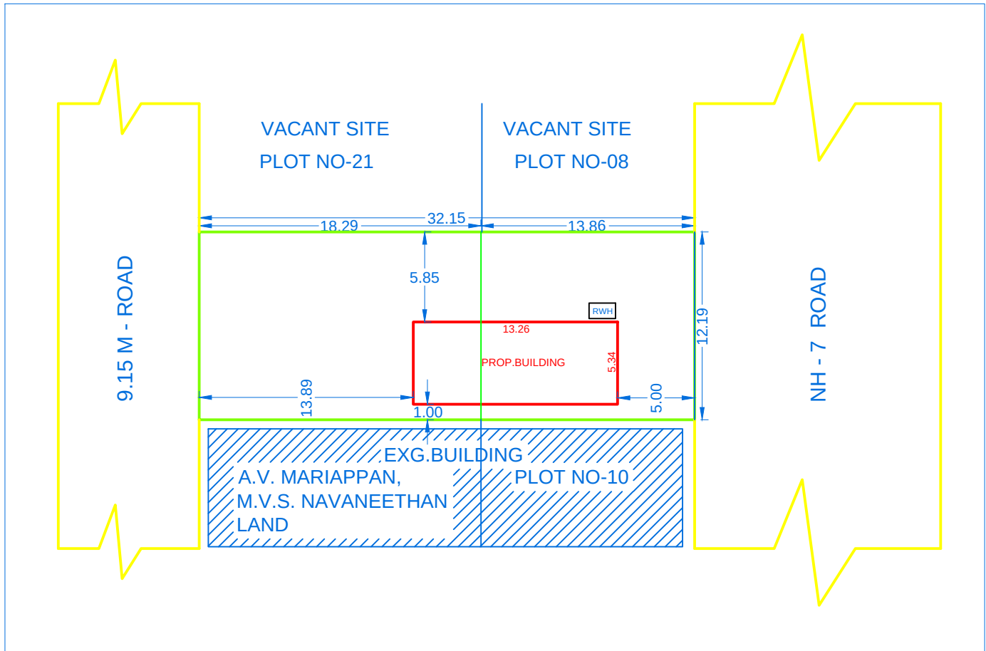
LOCATION PLAN Scale 1:400
