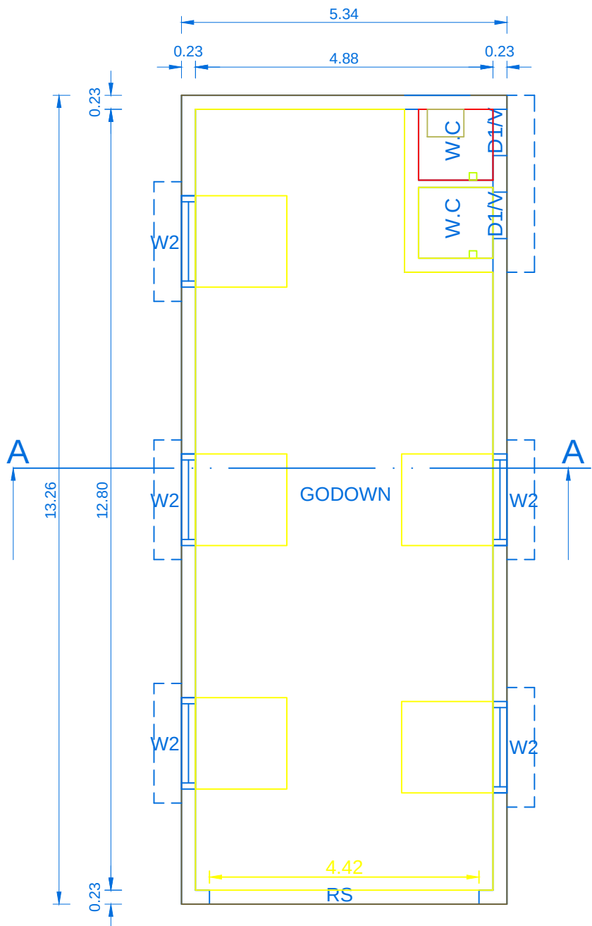
FLOOR PLAN
