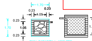
DETAILS OF FILTER BED & WELL
