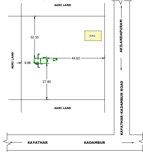
SITE PLAN
