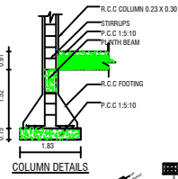
COLUMN DETAILS
