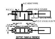
SEPTIC TANK & TRENCH
