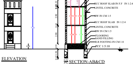
SECTION-AB&CD
