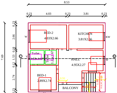
PRO.F.FLOOR PLAN
