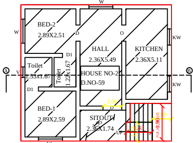
EXG.G.FLOOR PLAN
