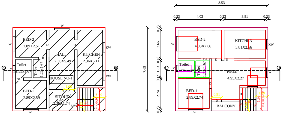
EXG.G.FLOOR PLAN
