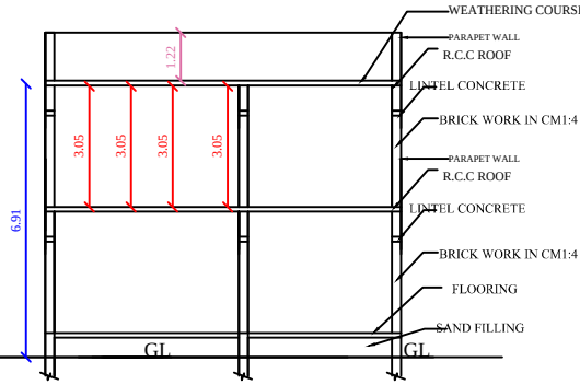
SECTION ON AB&CD
