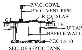
SEC. OF SEPTIC TANK
