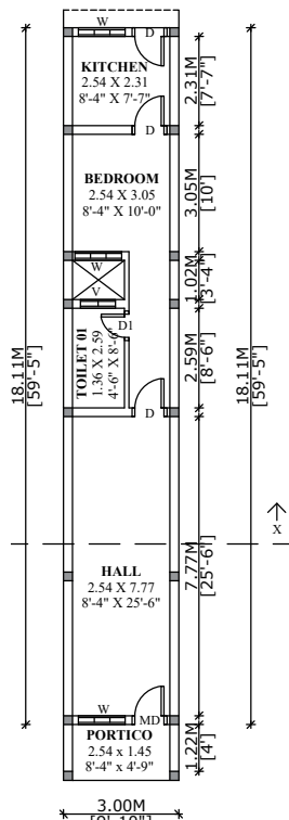
ROUND FLOOR PLAN
