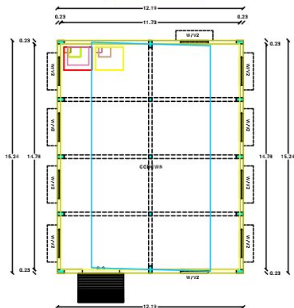
PLAN (GODOWN)
