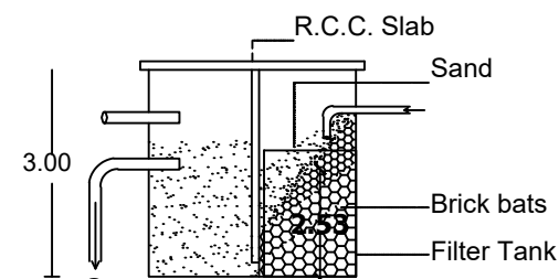
RAINWATER HARVESTING
