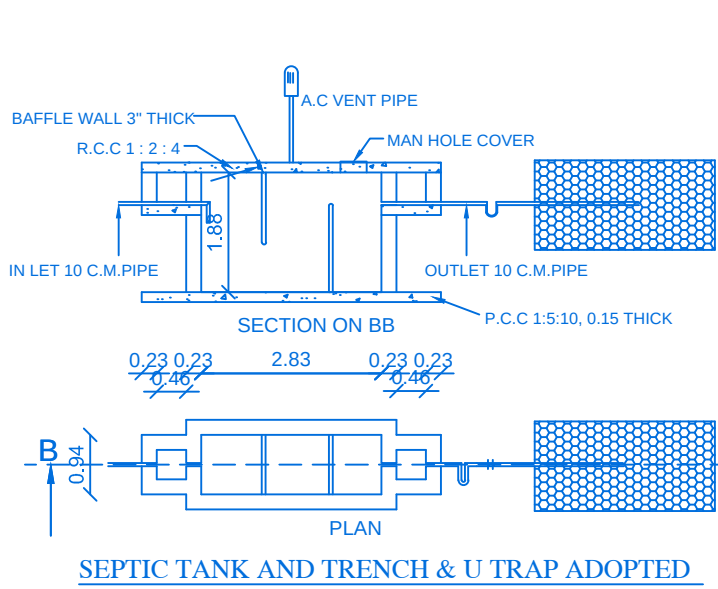
SEPTIC TANK AND TRENCH & U TRAP ADOPTED
