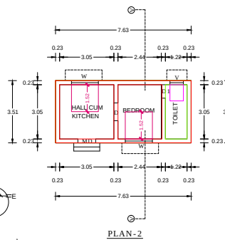
PLAN - 2
