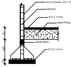
COLUMN DETAIL
