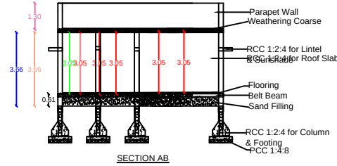
SECTION AB
