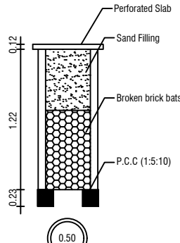
RAIN WATER COLLECTION WELL
