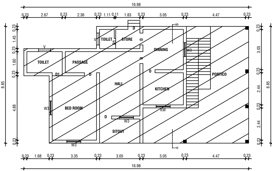
EXG GROUND FLOOR PLAN
