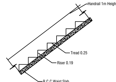
STAIR DETAILS
