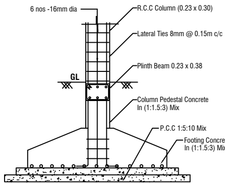
COLUMN FOOTING DETAILS
