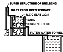
RAINWATER HARVESTING
