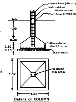
Details of COLUMN
