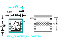
DETAILS OF FILTER BED & WELL
