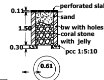
percolation pit
