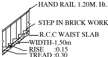
STAIR DETAIL
