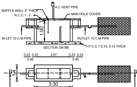
SEPTIC TANK AND TRENCH & U TRAP ADOPTED
