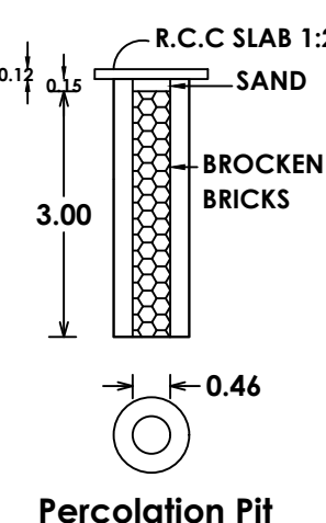
Percolation Pit
