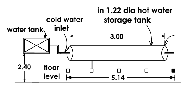
Details Of Solar Water Heating System
