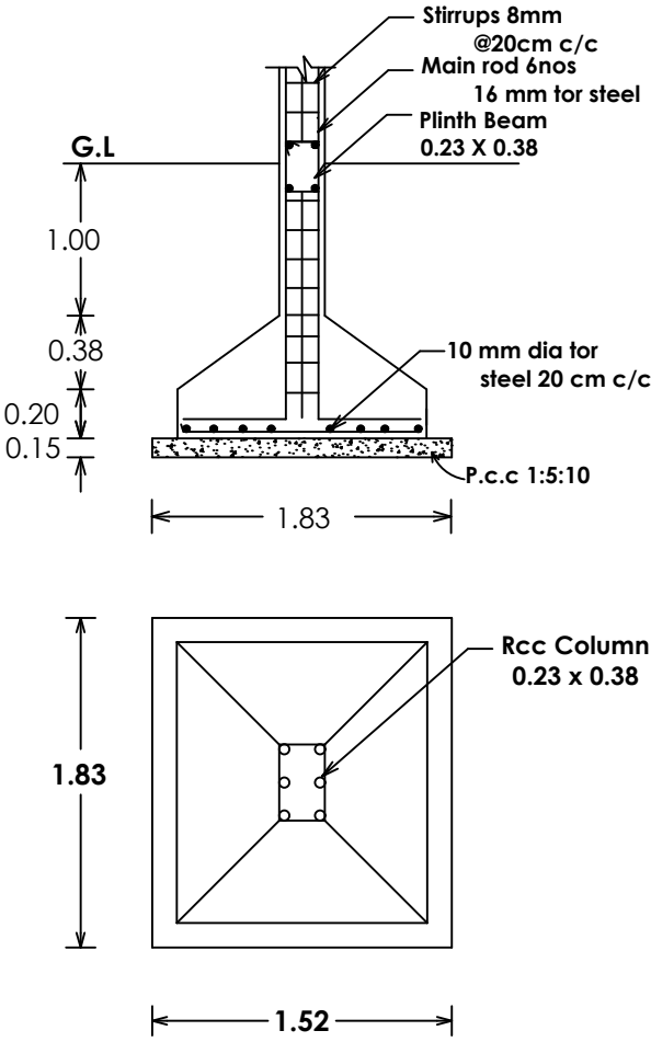
Details of Column Footing
