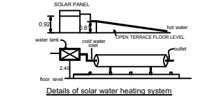
Details of solar water heating system
