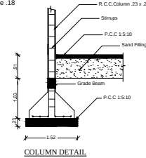
COLUMN DETAIL
