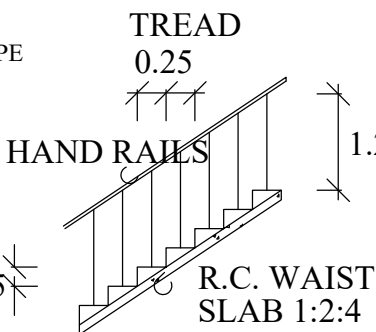
STAIRCASE DETAIL
