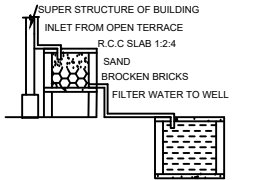
RAINWATER HARVESTING
