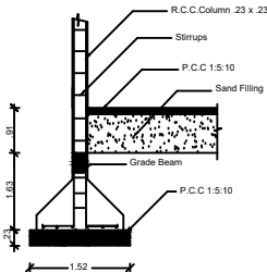
COLUMN DETAIL
