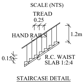
STAIRCASE DETAIL
