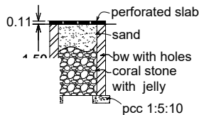
Foundation pit
