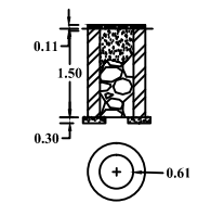
PERCOLATION PIT
