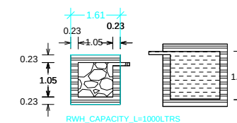
DETAILS OF FILTER BED & WELL
