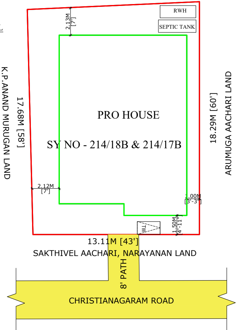
SITE PLAN
