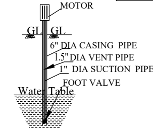
SEC. OF BOREWELL
