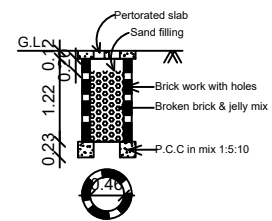
PERCOLATION PIT FOR 30 Sq.m (Scale:- 1:50)
