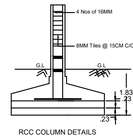
RCC COLUMN DETAILS
