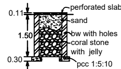
Percolation pit
