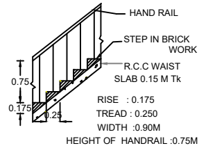
STAIR DETAILS
