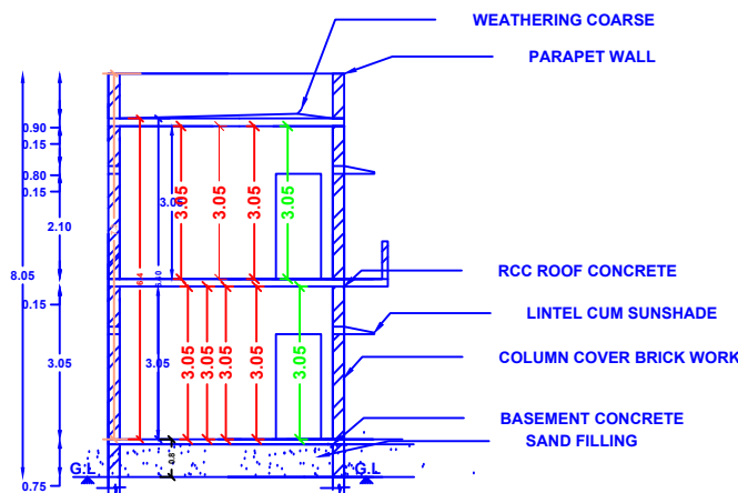
SECTION AB
