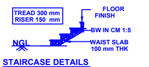
STAIRCASE DETAILS
