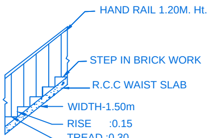
STAIR DETAIL
