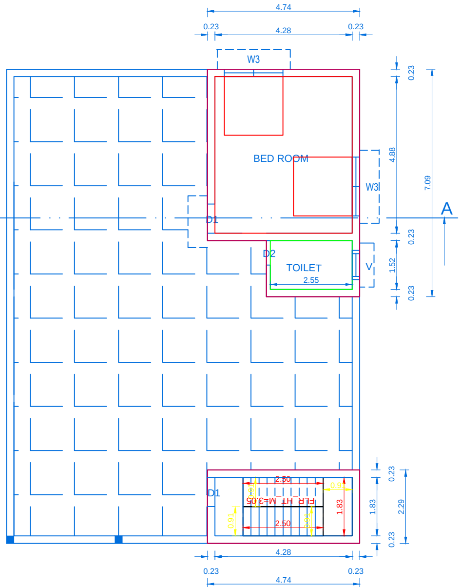
PROP.SECOND FLOOR PLAN
