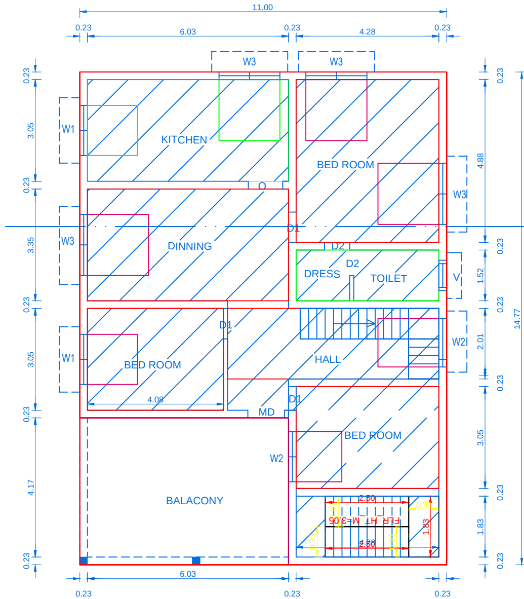
EXG & PROP.FIRST FLOOR PLAN
