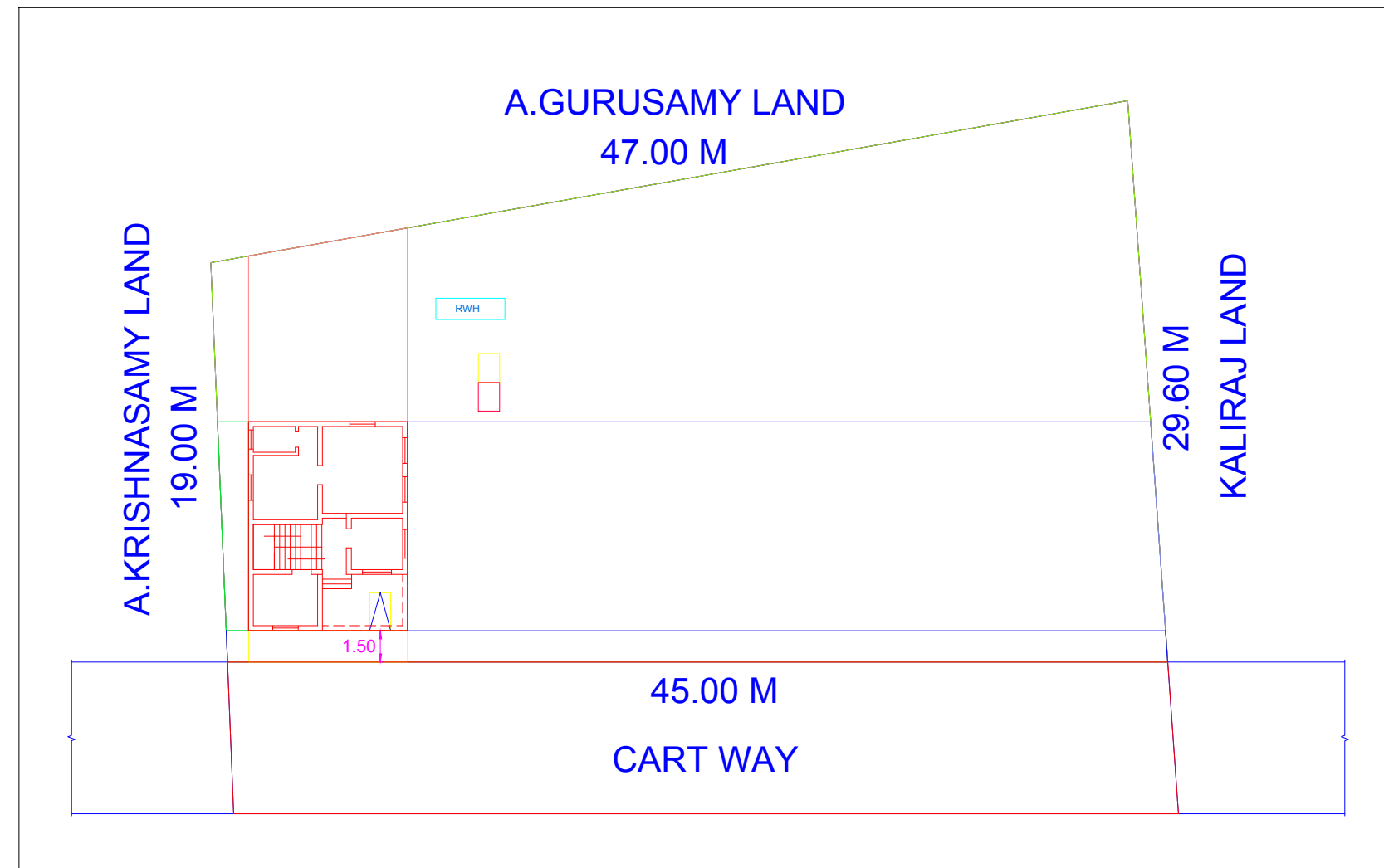
AREA DETAILS AREA DETAIL SQ.MT SQ.FT AREA OF SITE 1011.70 10890.00 GROUND FLOOR AREA OF BUILDING 74.90 806.22
