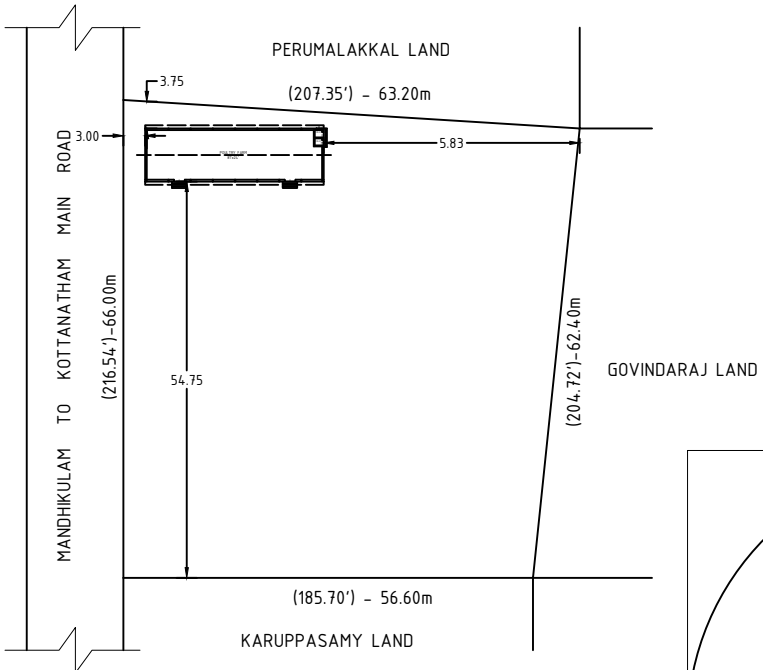
SITE PLAN SCALE (NTS)
