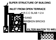
SUPER STRUCTURE OF BUILDING
