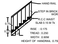
STAIR DETAILS
